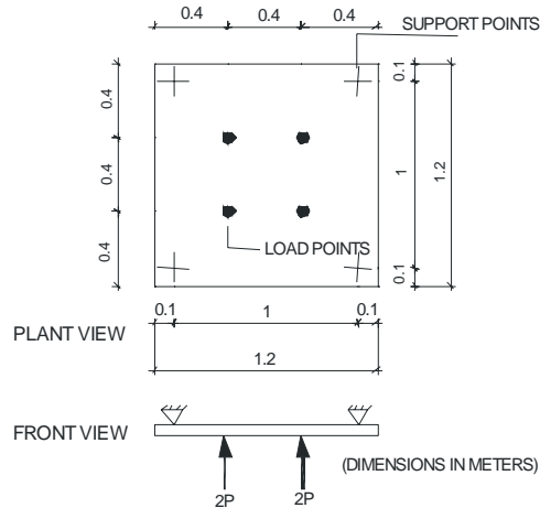
Figure 2: Second load system.
