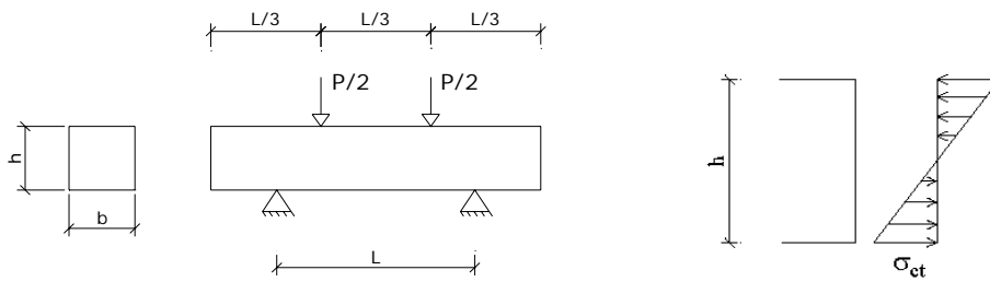
Figure 5 – Behavior of the central area in the specimen before cracking.
